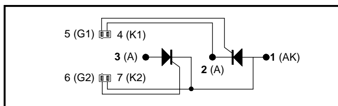
Fig. 1 TT Circuit diagram
