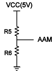
Figure 5: AAM Network
