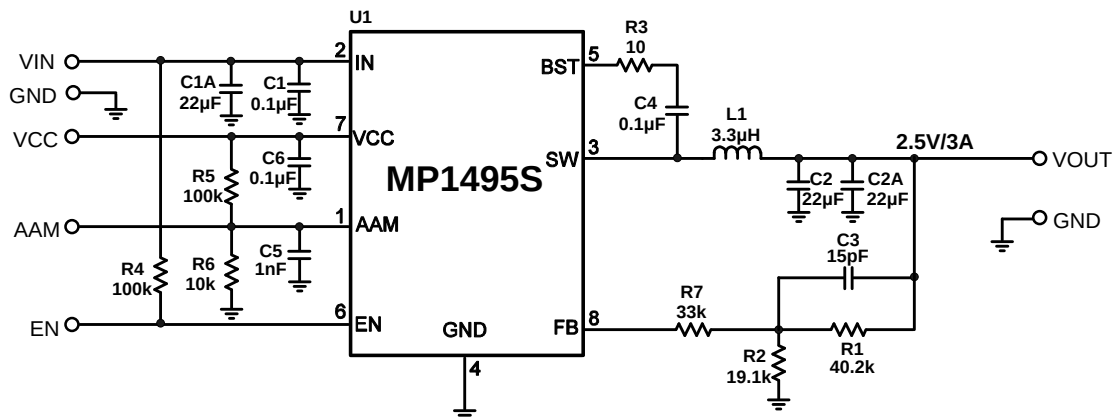
Figure 9: 12V IN , 2.5V/3A Output
