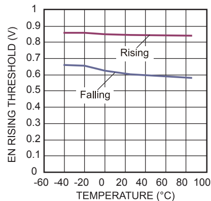
EN Rising and Falling Threshold vs. Temperature
