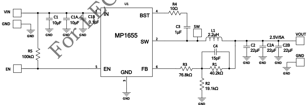
Figure 8: V_{IN} = 12V , V_{OUT} = 2.5V/5A
