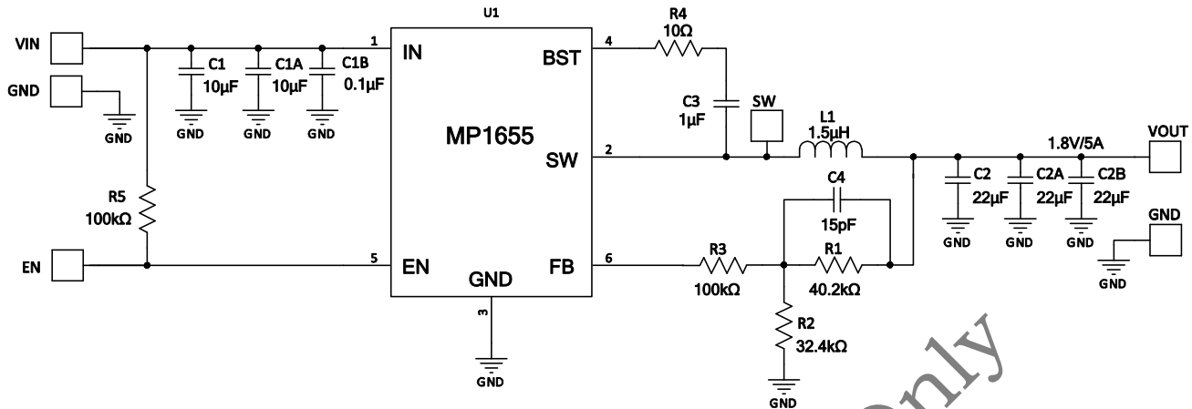
Figure 9: V_{IN} = 12V , V_{OUT} = 1.8V/5A
