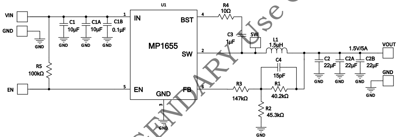
Figure 10: V_{IN} = 12V , V_{OUT} = 1.5V/5A
