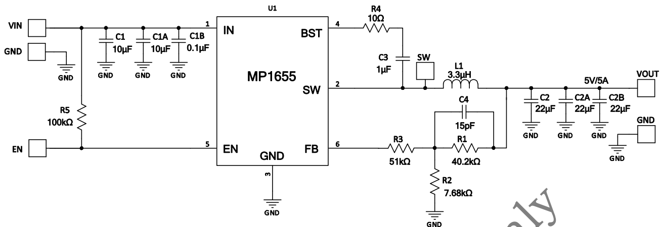
Figure 6: V_{IN} = 12V , V_{OUT} = 5V/5A
