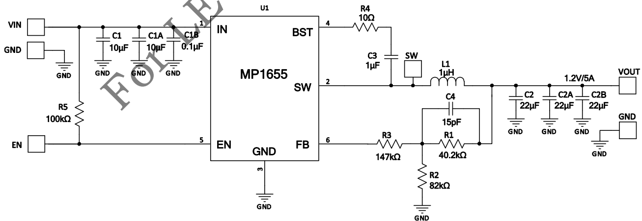
Figure 11: V_{IN} = 12V , V_{OUT} = 1.2V/5A
