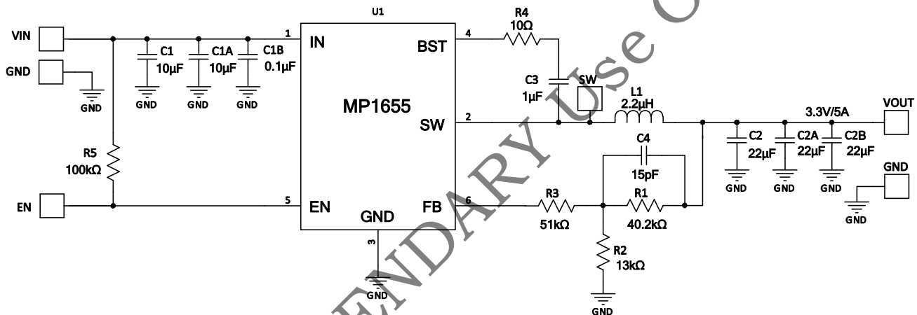
Figure 7: V_{IN} = 12V , V_{OUT} = 3.3V/5A
