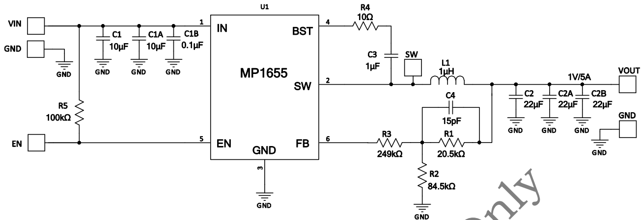
Figure 12: V_{IN} = 12V , V_{OUT} = 1V/5A
