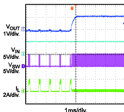
Short-Circuit Recovery
