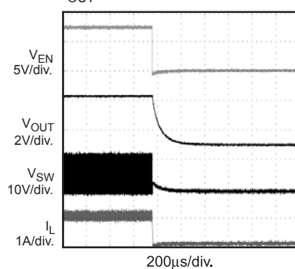
Shut-down through Enable I_{OUT} = 1A Resistive Load
