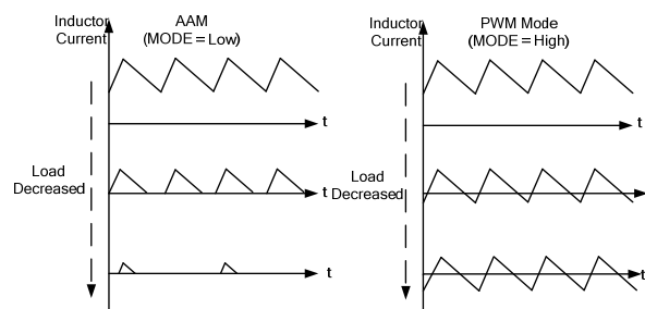
Figure 2: AAM and PWM Mode
