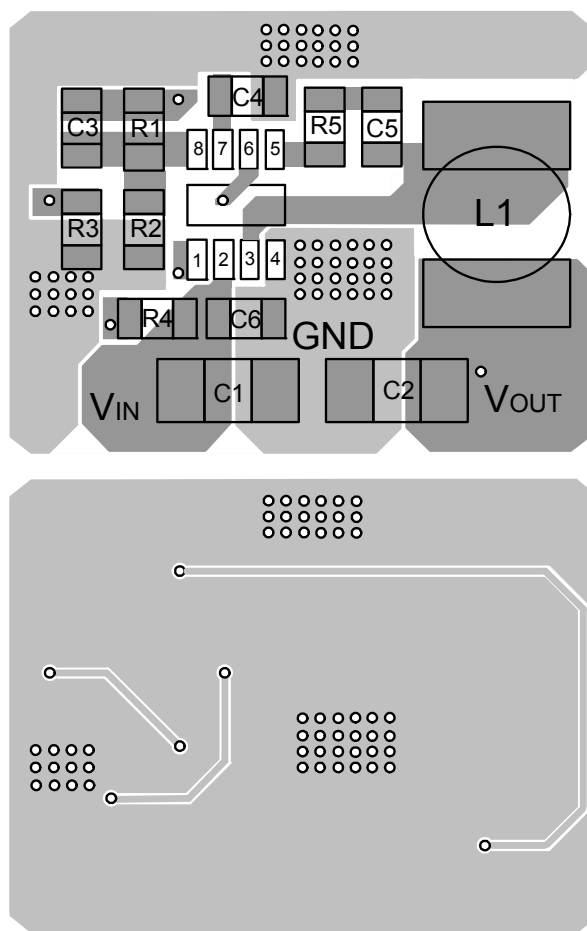
Figure 9: Sample Board Layout
