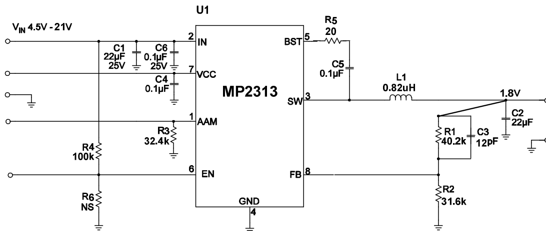
Figure 13: V_{IN}=12V , V_{OUT}=1.8V , I_{OUT}=1A
