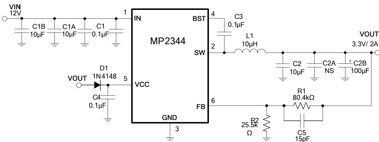
Figure 8: 3.3V/2A Output
