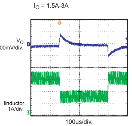
Loop Response
