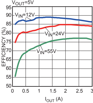
Efficiency vs. Output Current V OUT =5V
