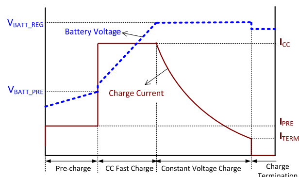
Figure 3 Charging Profile
