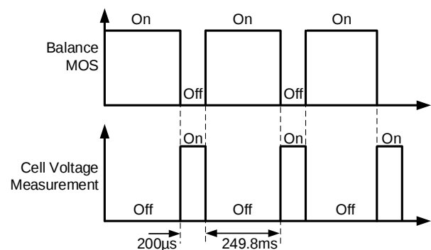
Figure 11: Battery Balance Clock
