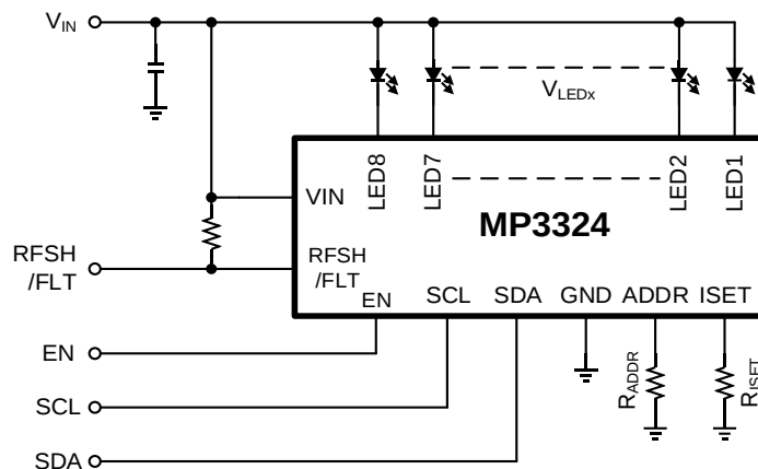
Figure 1: Typical Application
