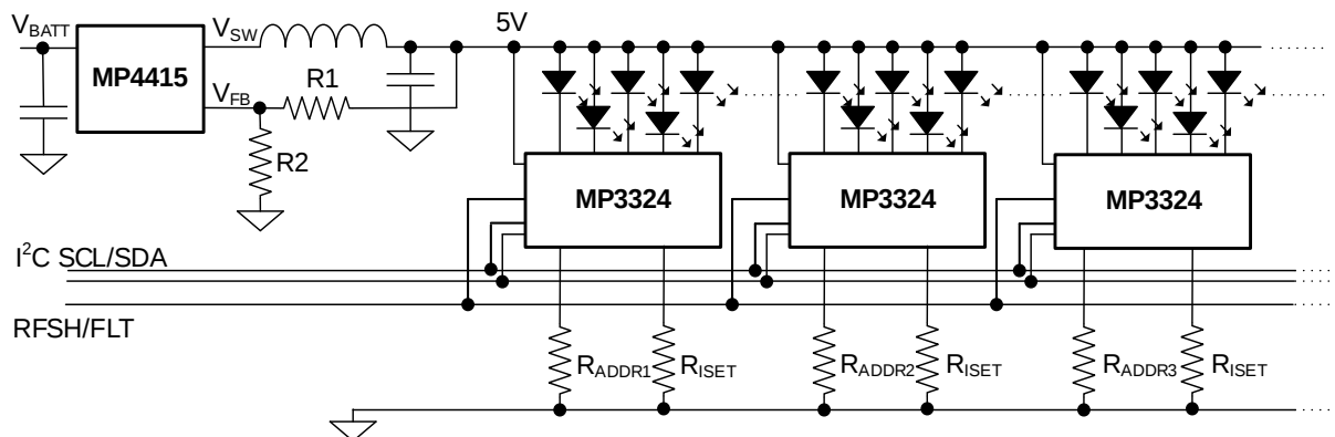
Figure 2: System Application
