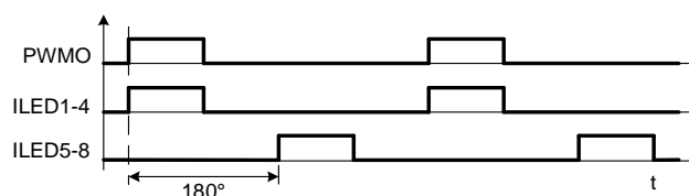
Figure 19: Phase Shift with 2 Channels
