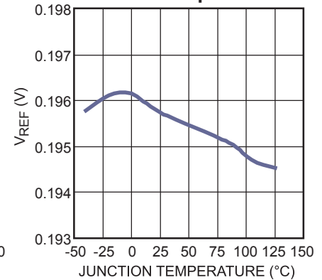
Feedback Reference vs. Junction Temperature
