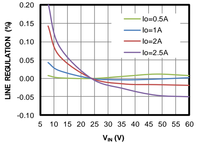
Line Regulation
