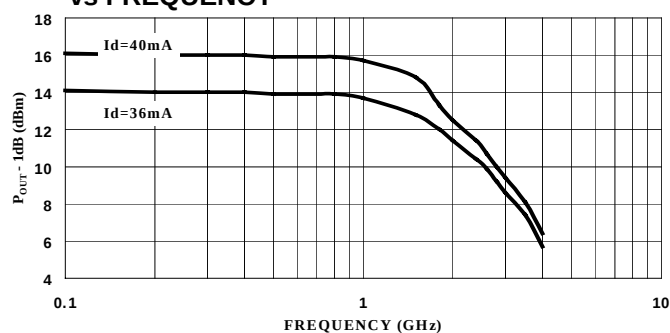
P_{OUT} @ 1dB GAIN COMPRESSION vs FREQUENCY
