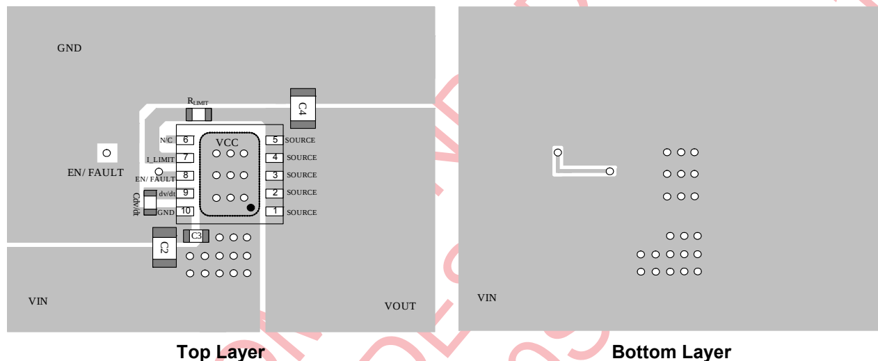
Figure 3—PCB Layout
