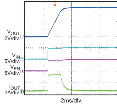
Start-Up through Input Voltage C_{OUT} = 2200\mu F
