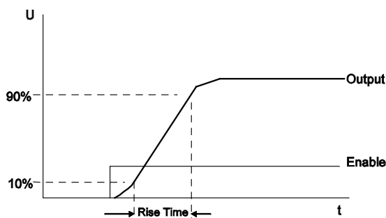
Figure 2: Rise Time
