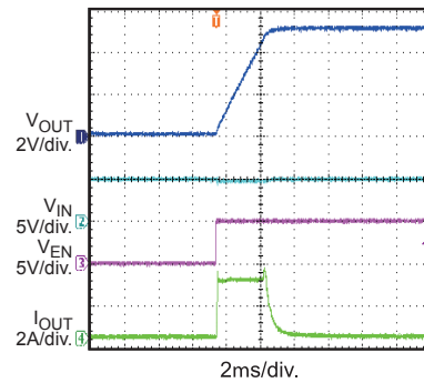
Start-Up through Enable/Fault C_{OUT} = 2200\mu F
