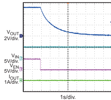
Shutdown through Enable/Fault No Load
