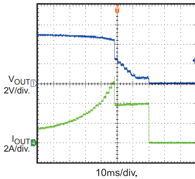
Current Limit
