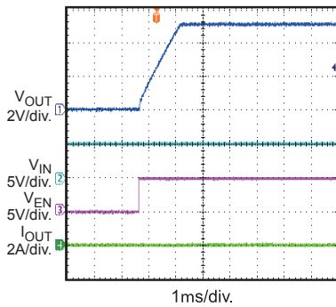
Start-Up through Enable/Fault No Load
