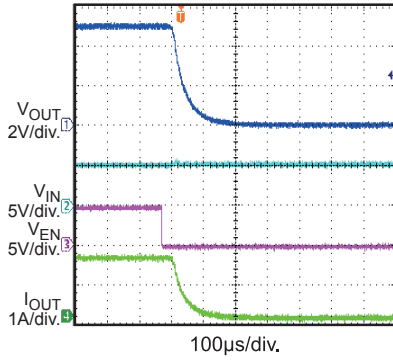
Shutdown through Enable/Fault R_{LOAD} = 3.3\Omega
