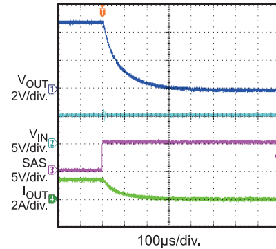
Shutdown through SAS R_{LOAD}=3.3\Omega
