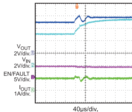
OVP Response
