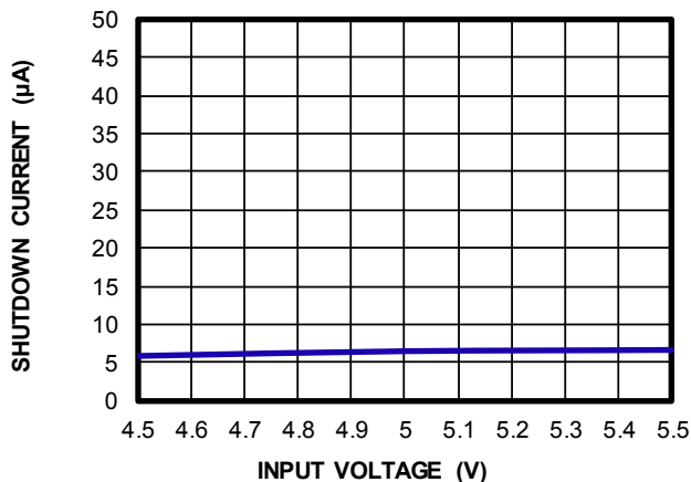
Shutdown Current vs. Input Voltage (5V E-Fuse)
