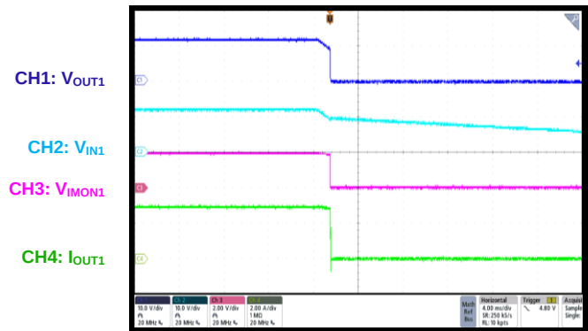
Shutdown through VIN1 12V e-fuse, 3A load
