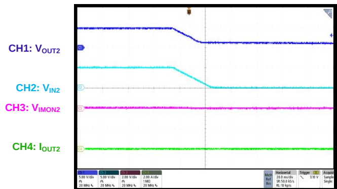
Shutdown through VIN2 5V e-fuse, no load
