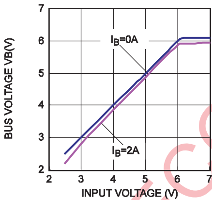
VB Bus Clamping Voltage
