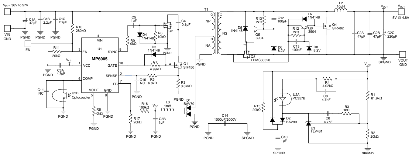
Figure 16: Typical SSR Forward Application Circuit (16)
