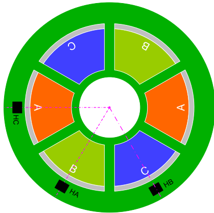
Figure 10: Hall Sensor Placement Option 1
