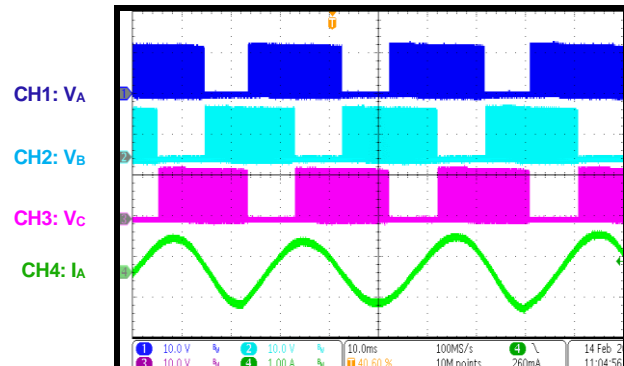
Steady State PWM duty = 50%, DIR = high, CW
