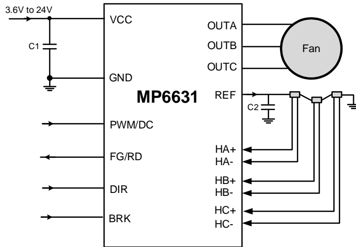
Figure 1: Triple Hall-Effect Sensor Application
