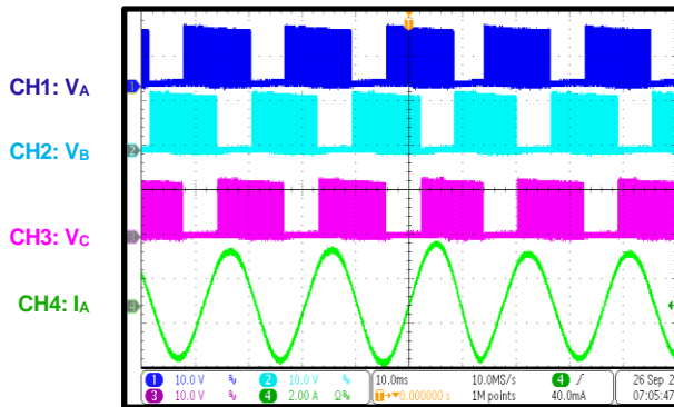
Steady State PWM duty = 100%, DIR = high, CW
