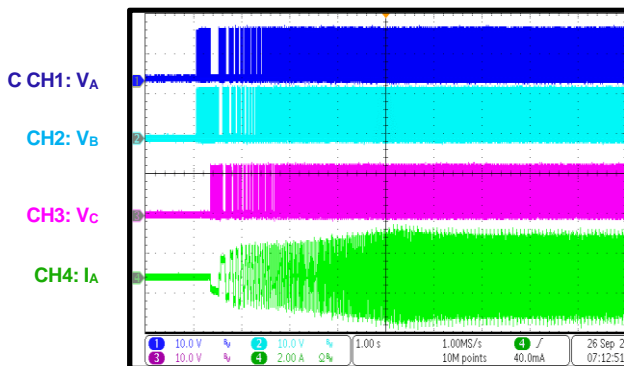
PWM On PWM duty = 0% to 100%, triple Hall-effect sensor, DIR = low, CCW
