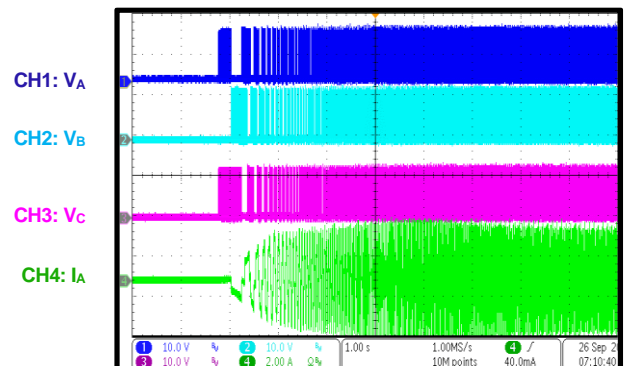
PWM On PWM duty = 0% to 100%, triple Hall-effect sensor, DIR = high, CW
