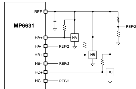
Figure 9: Hall-Sensor IC Connection
