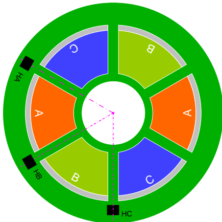
Figure 11: Hall Sensor Placement Option 2
