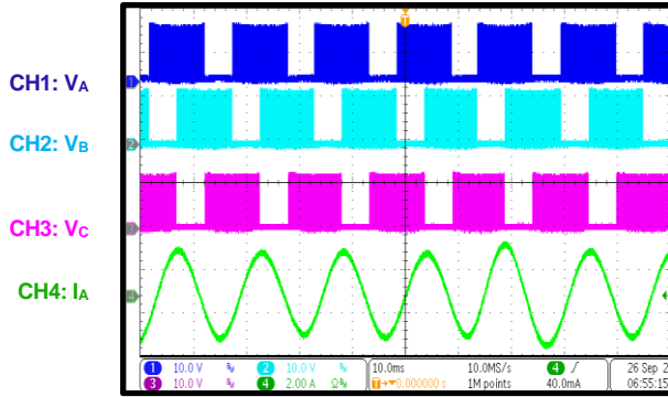
Steady State PWM duty = 100%, DIR = low, CCW
