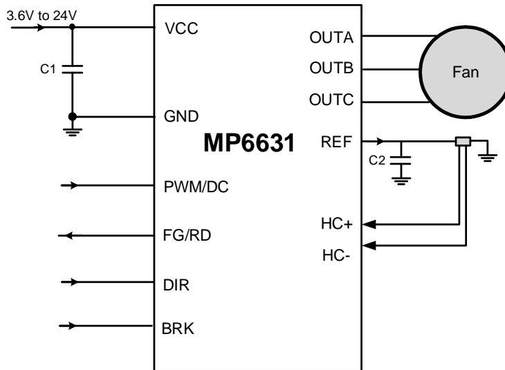
Figure 2: Single Hall-Effect Sensor Application
