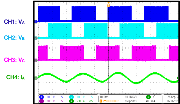
Steady State PWM duty = 50%, DIR = low, CCW
