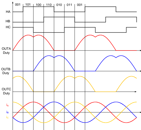
Figure 4: MP6631 Hall Output and Output Drive
