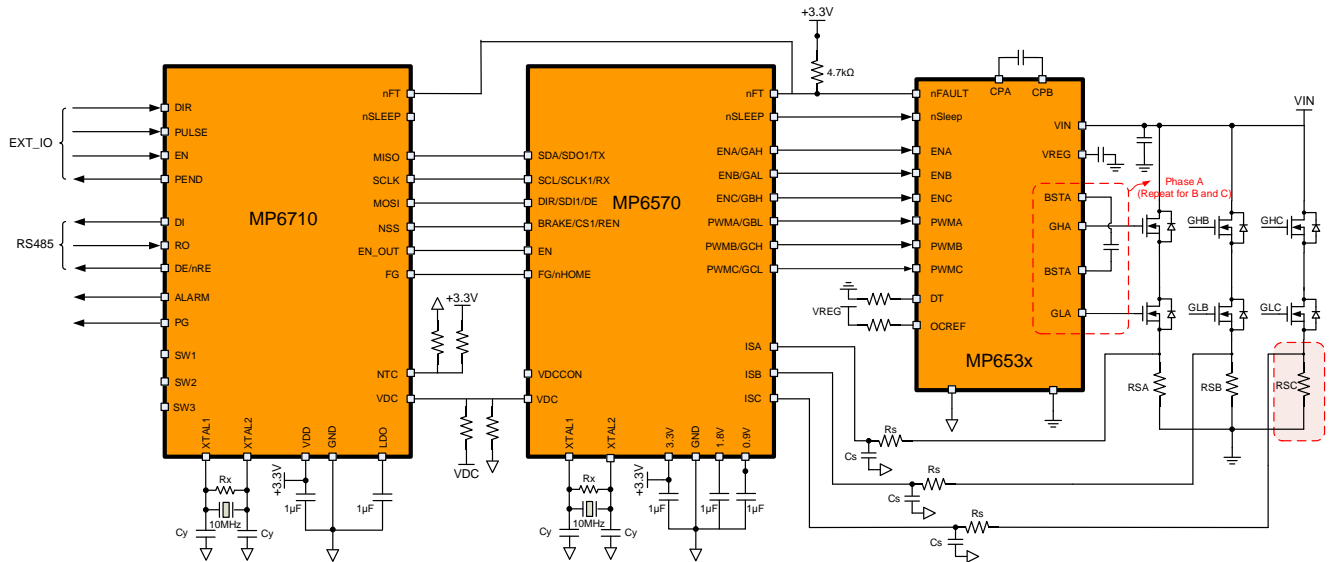
Figure 2: MP6710 + MP6570 + Pre-Driver + MOSFETs Solution
