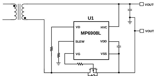
Figure 5: Low-Side Rectification
