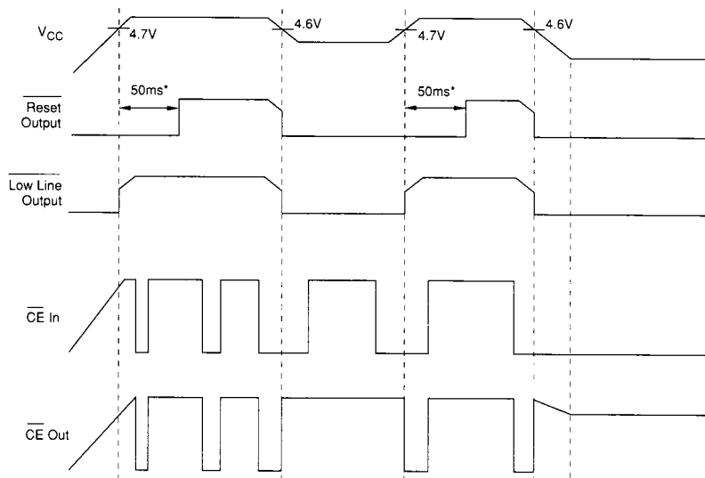
Figure 6. Reset Timing
