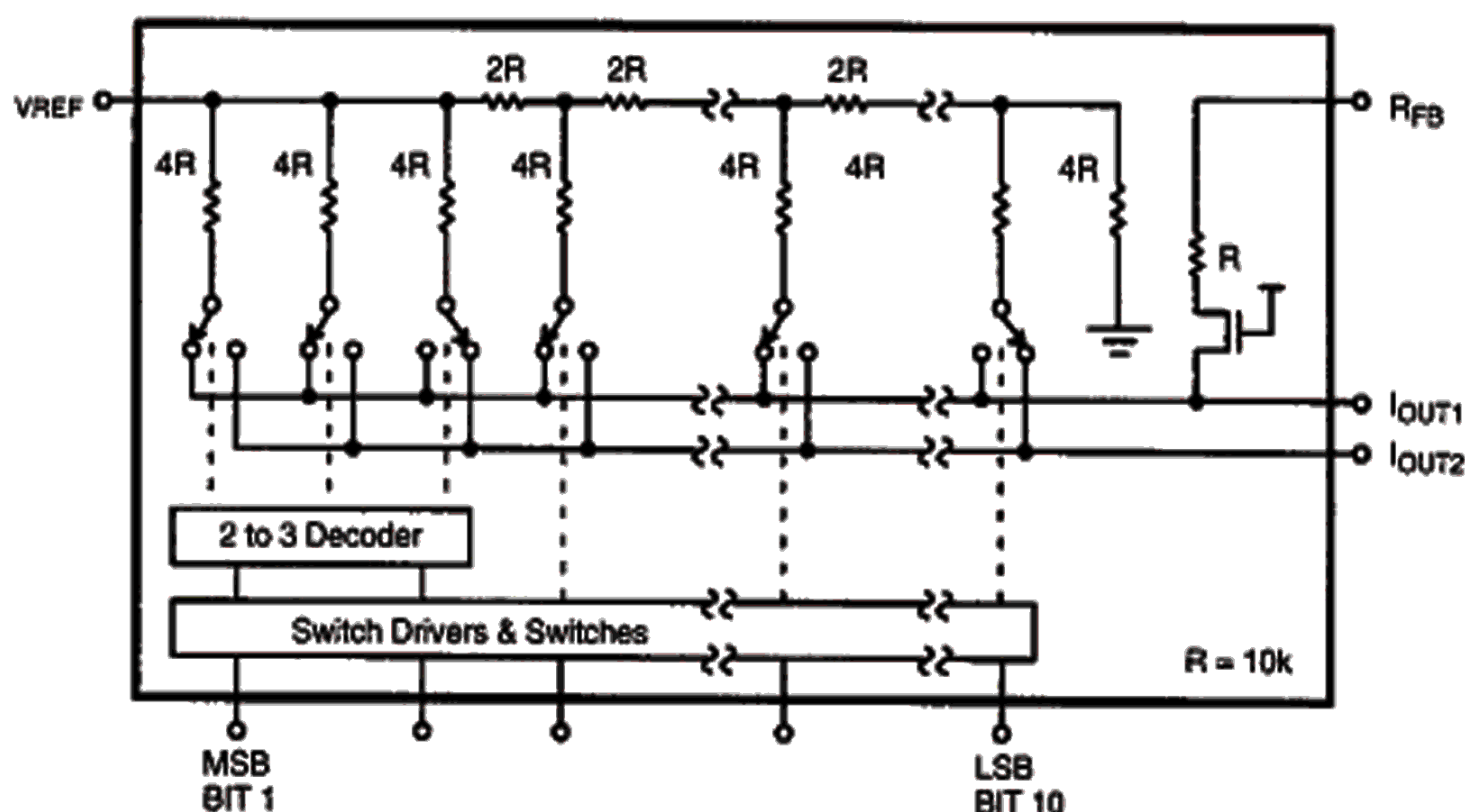
3 Segment D/A Converter with Termination to GND. Logical "1" at Digital Input Steers Current to I_{\text{OUT}1}
