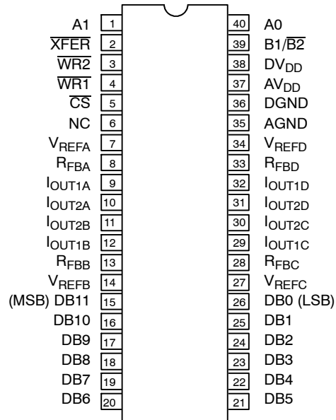
40 Pin PDIP , (0.600 )
