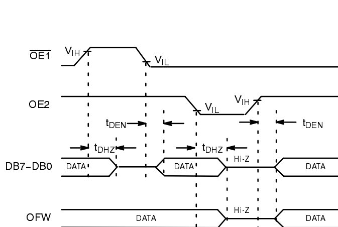
Figure 2. Output Enable/Disable Timing Diagram
