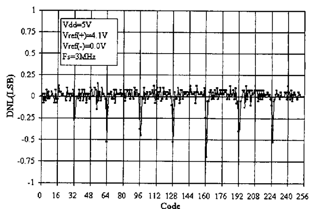
Graph 14. DNL Error Plot
