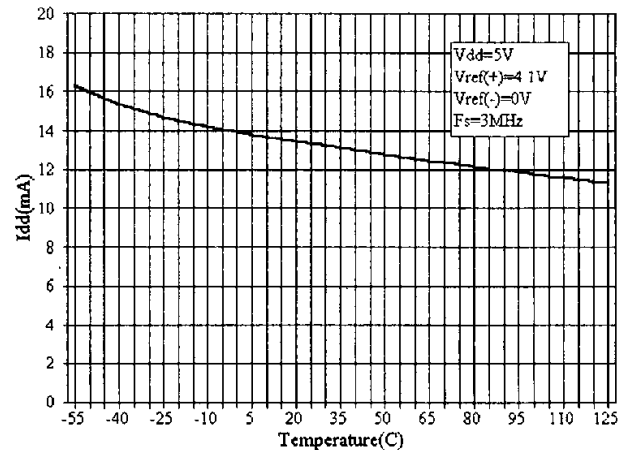
Graph 6. Supply Current vs. Temperature
