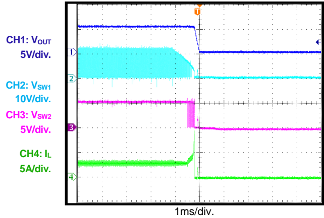
V_{IN} Power Off Load = 3A
