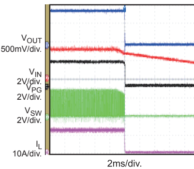
Shutdown through Input Voltage I_{OUT} = 12A
