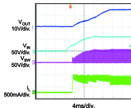
Power On I_{OUT} = 300mA
