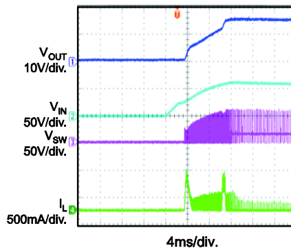
Power On I_{OUT} = 5mA
