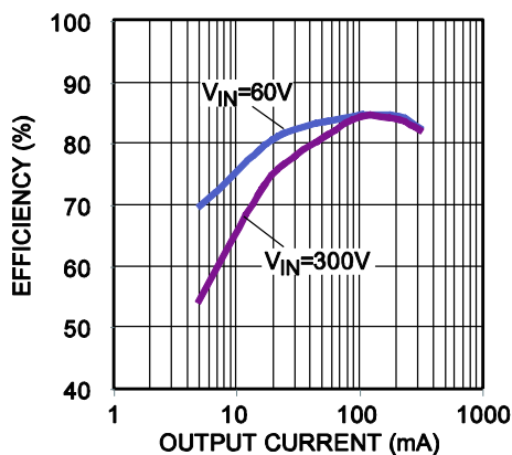
Efficiency L = 1.2mH
