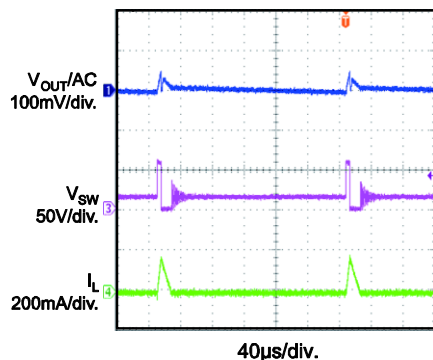
Steady State I_{OUT} = 5mA
