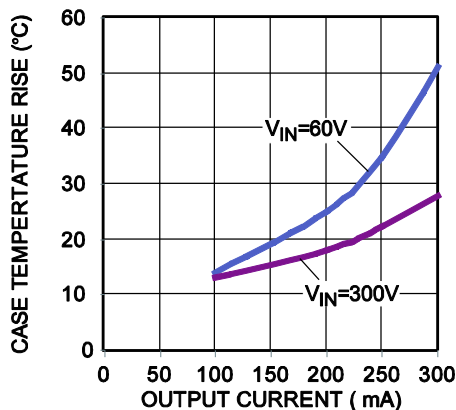
Case Temperature Rise
