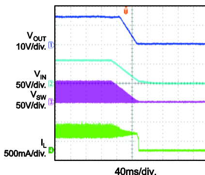
Power Off I_{OUT} = 300mA
