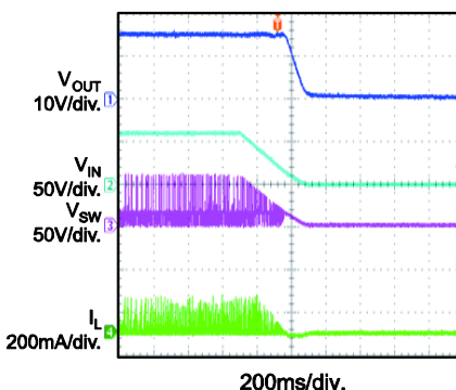
Power Off I_{OUT} = 5mA
