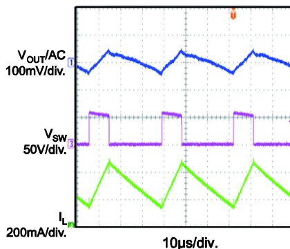
Steady State I_{OUT} = 300mA
