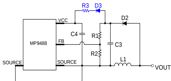
Figure 7: Auxiliary VCC Supply Circuit
