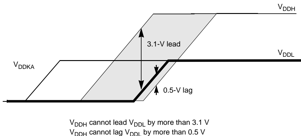
Figure F-2. Option A Power-Up Sequence With Keep-Alive Supply
