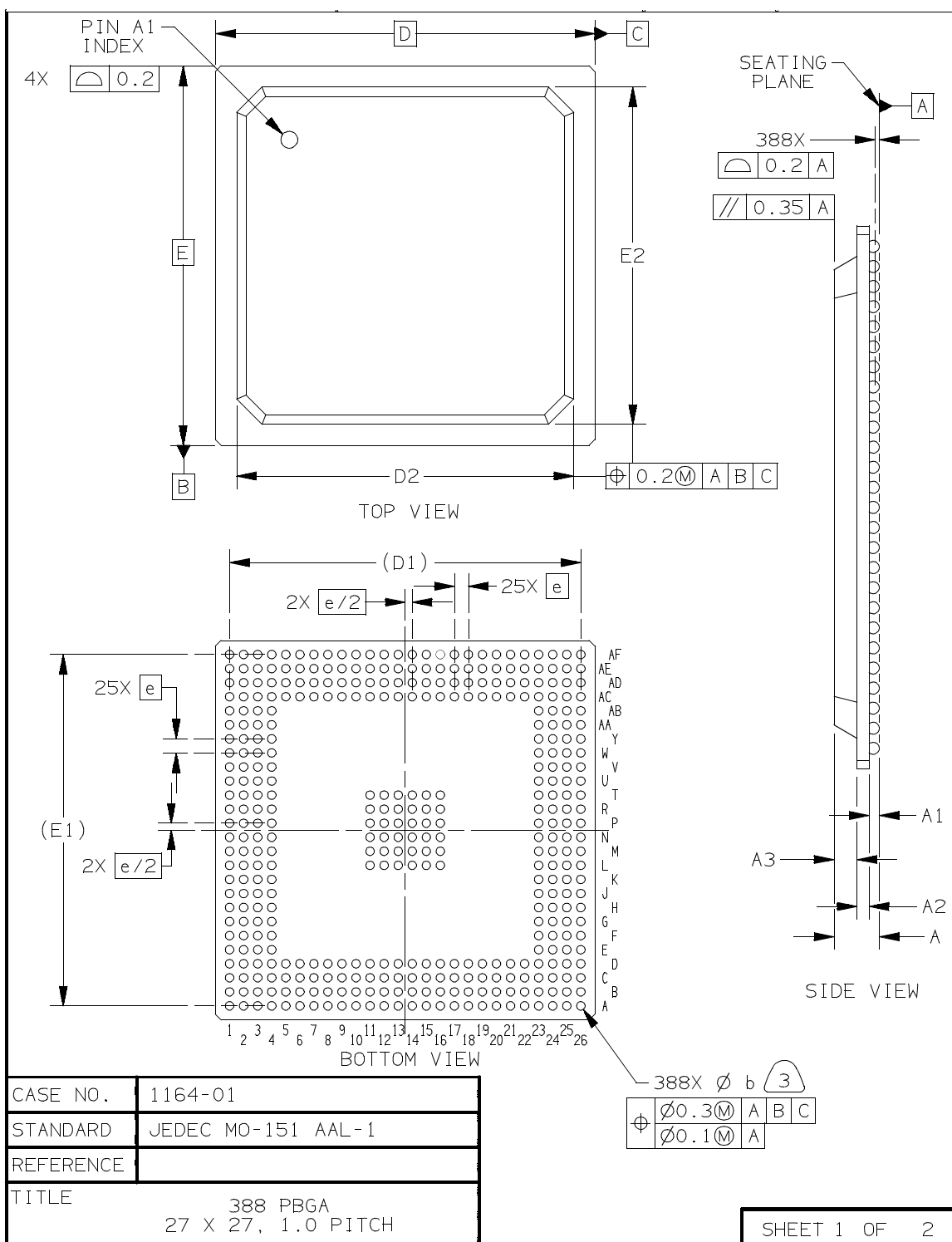
Figure G-63. MPC561/MPC563 Package Footprint (1 of 2)
