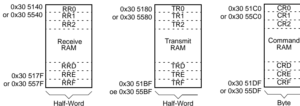
Figure 15-16. QSPI RAM
