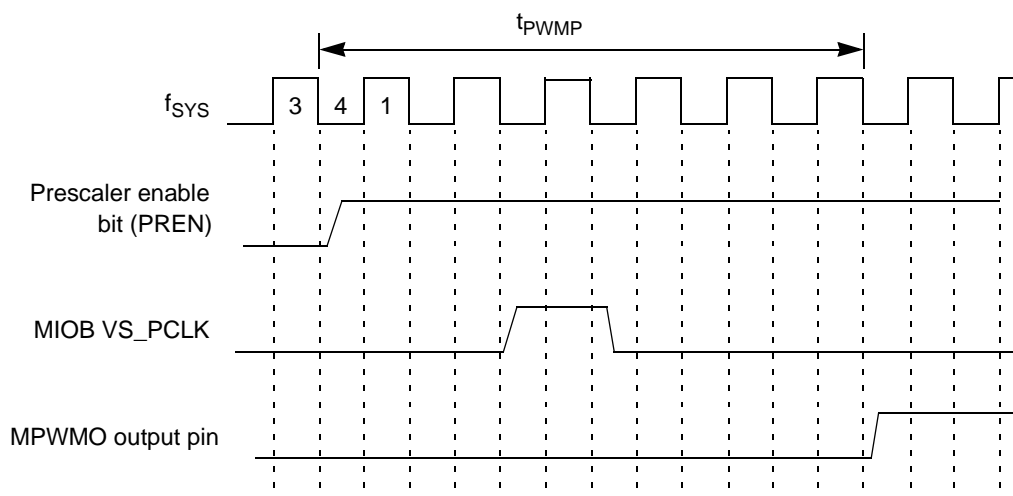
Figure F-49. MCPWM Enable to MPWMO Output Pin Rising Edge Timing Diagram
