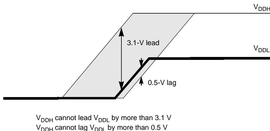
Figure F-1. Option A Power-Up Sequence Without Keep-Alive Supply
