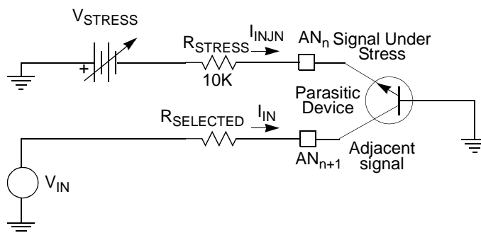
Figure 13-54. Input Signal Subjected to Negative Stress
