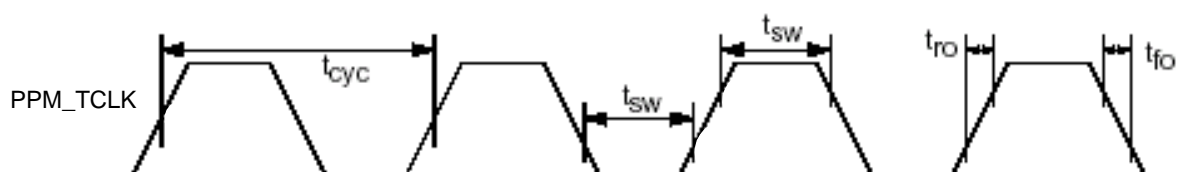
Figure G-44. PPM_TCLK Timing
