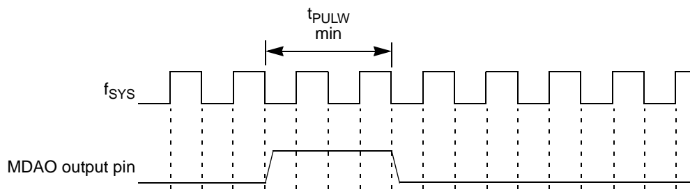
Figure G-59. MDASM Minimum Output Pulse Width Timing Diagram
