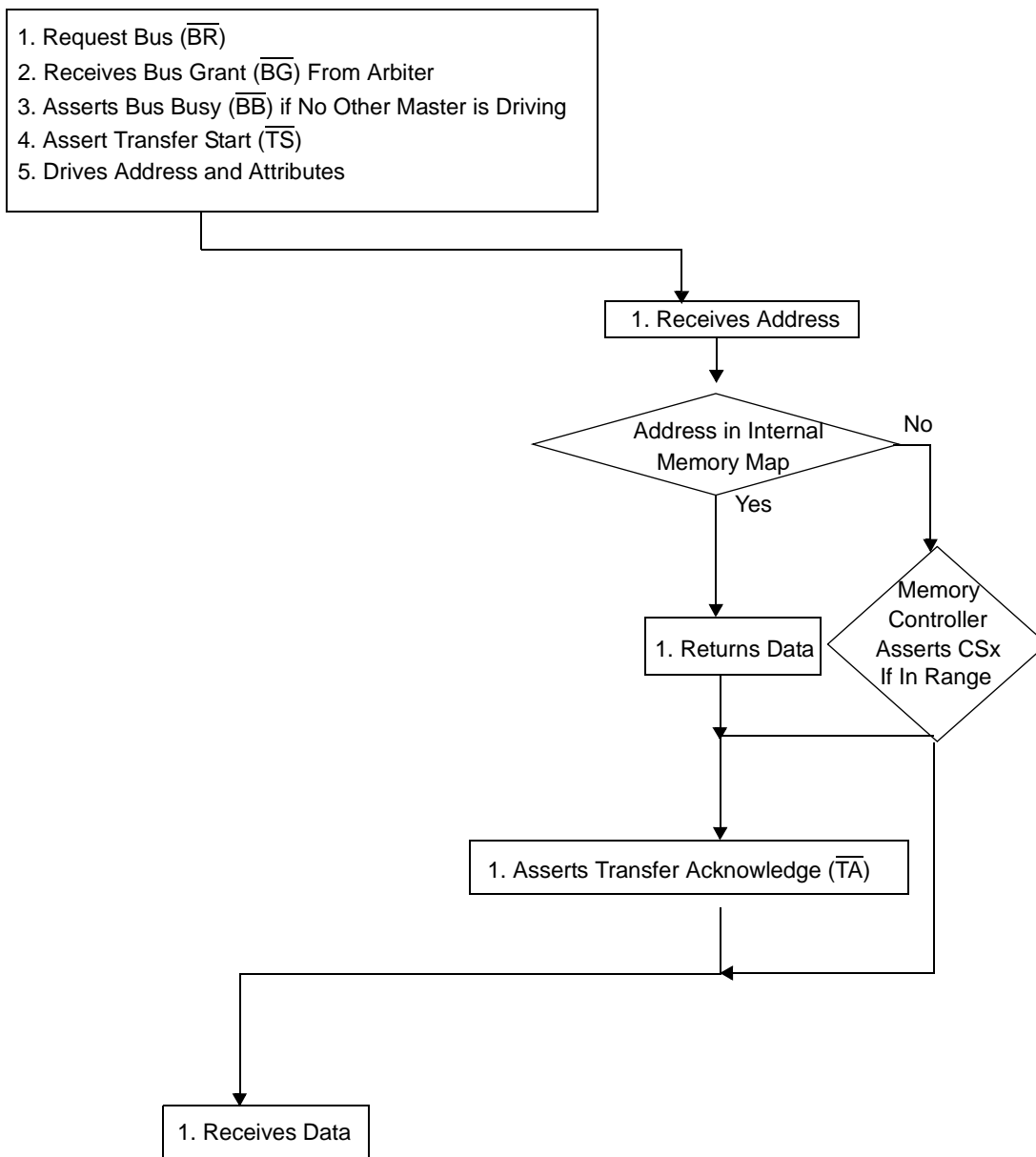
Figure 9-35. Basic Flow of an External Master Read Access
