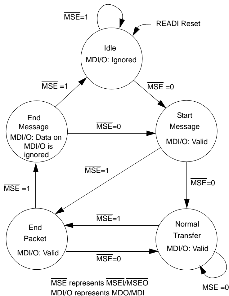
Figure 24-13. MSEI/MSEO Transfers
