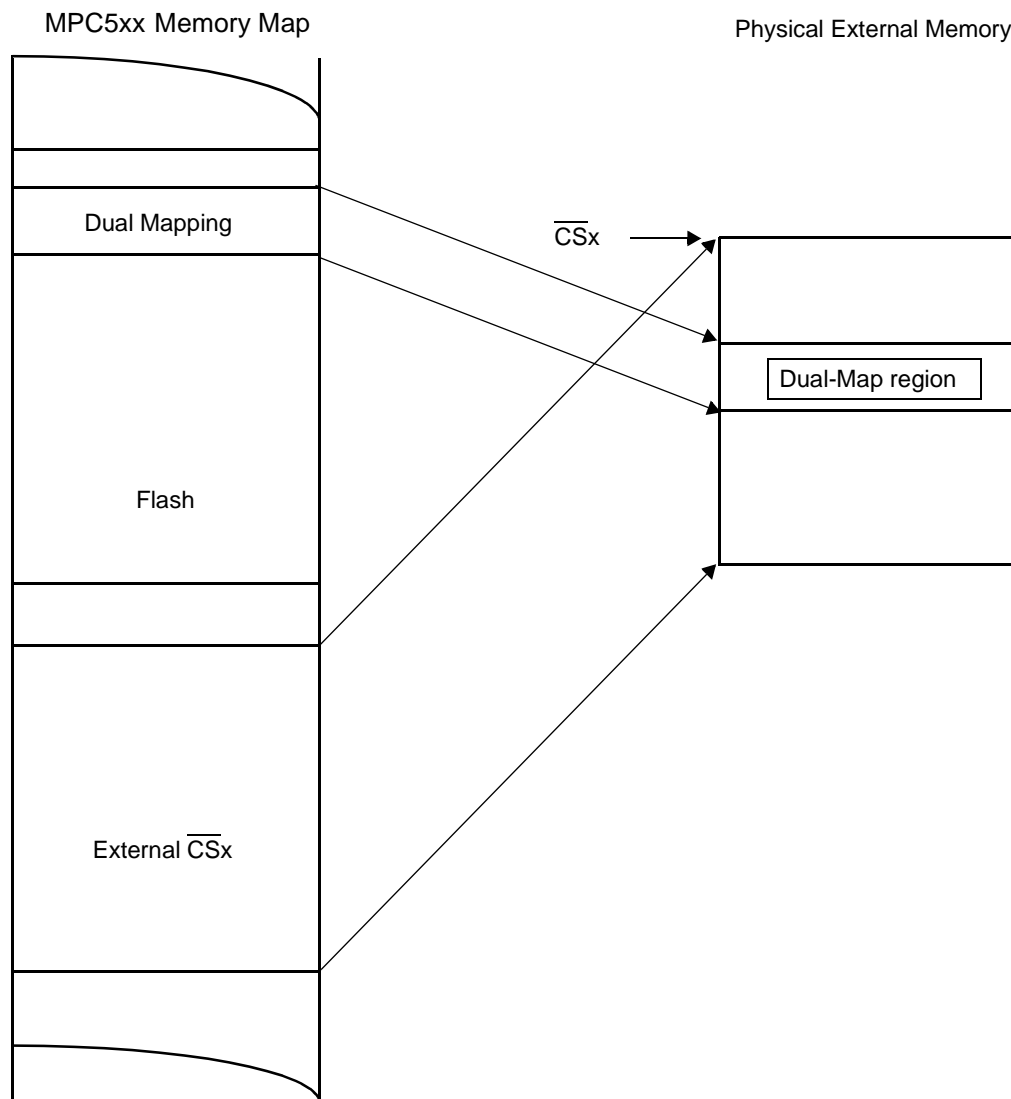
Figure 10-19. Aliasing Phenomenon Illustration
