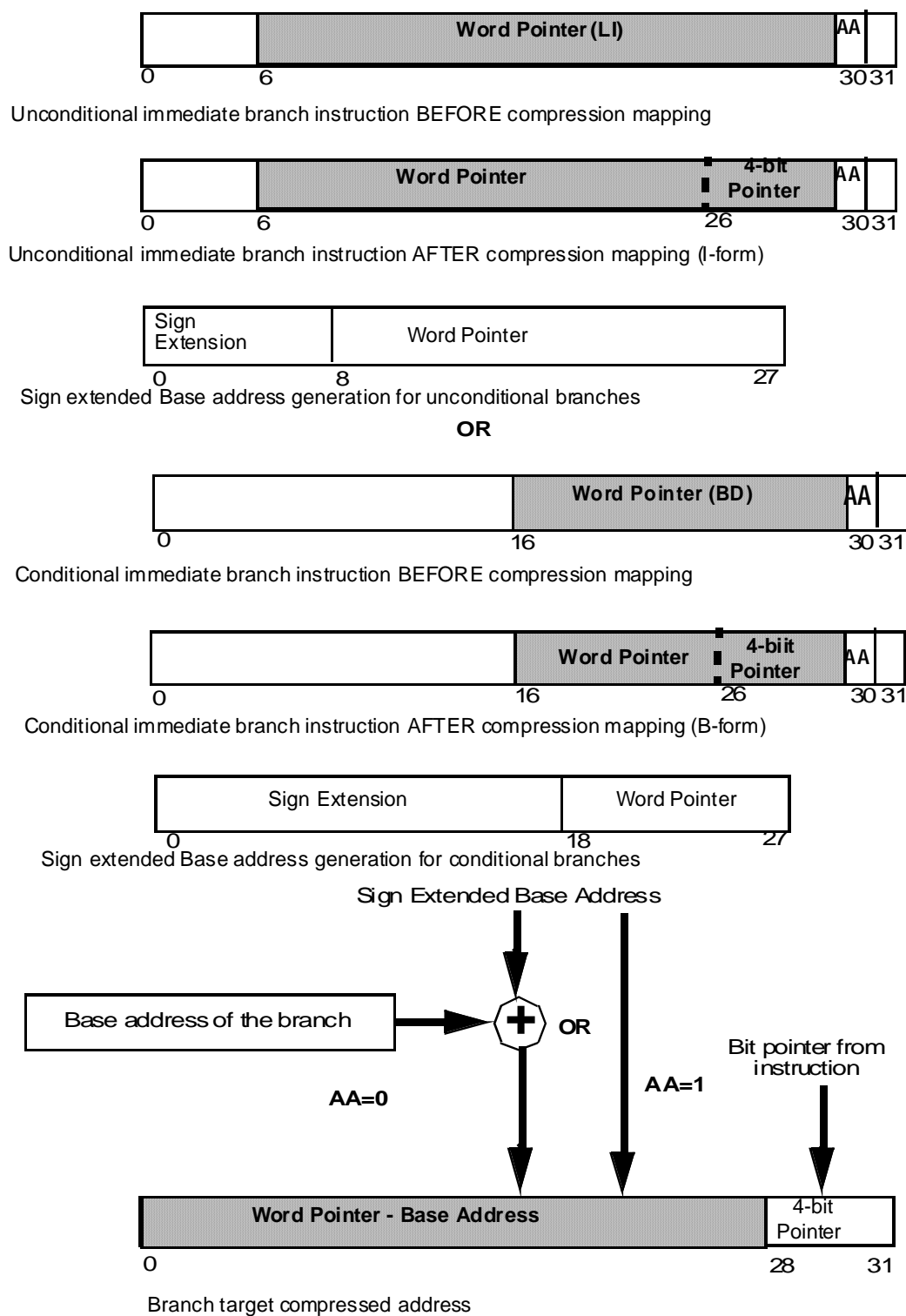
Figure A-3. Compressed Target Address Generation by Direct Branches
