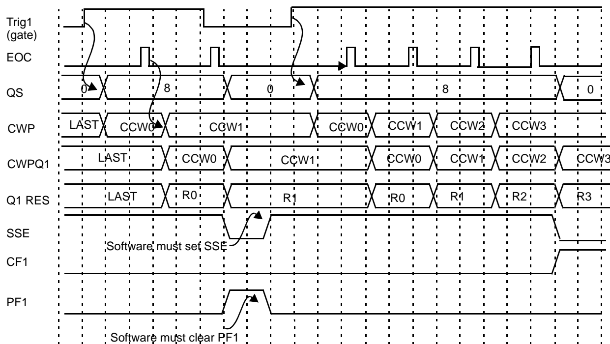
Figure 14-45. Gated Mode, Single-Scan Timing
