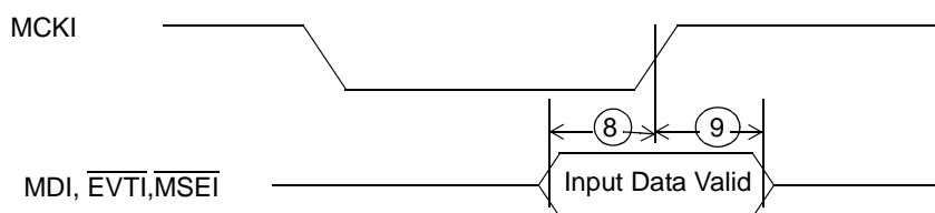
Figure F-30. Auxiliary Port Data Input Timing Diagram
