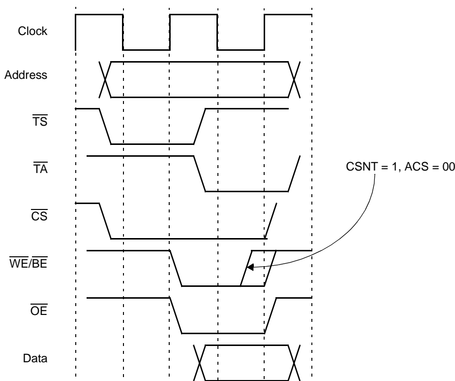
Figure 10-8. Memory Devices Interface Basic Timing (ACS = 00, TRLX = 0)
