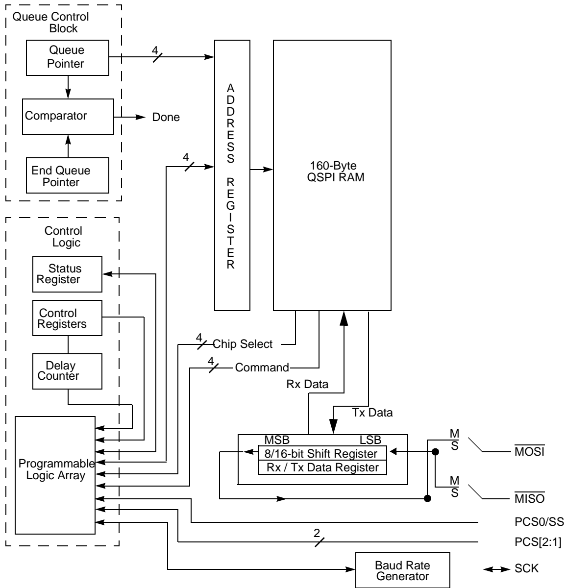
QSPI Block
