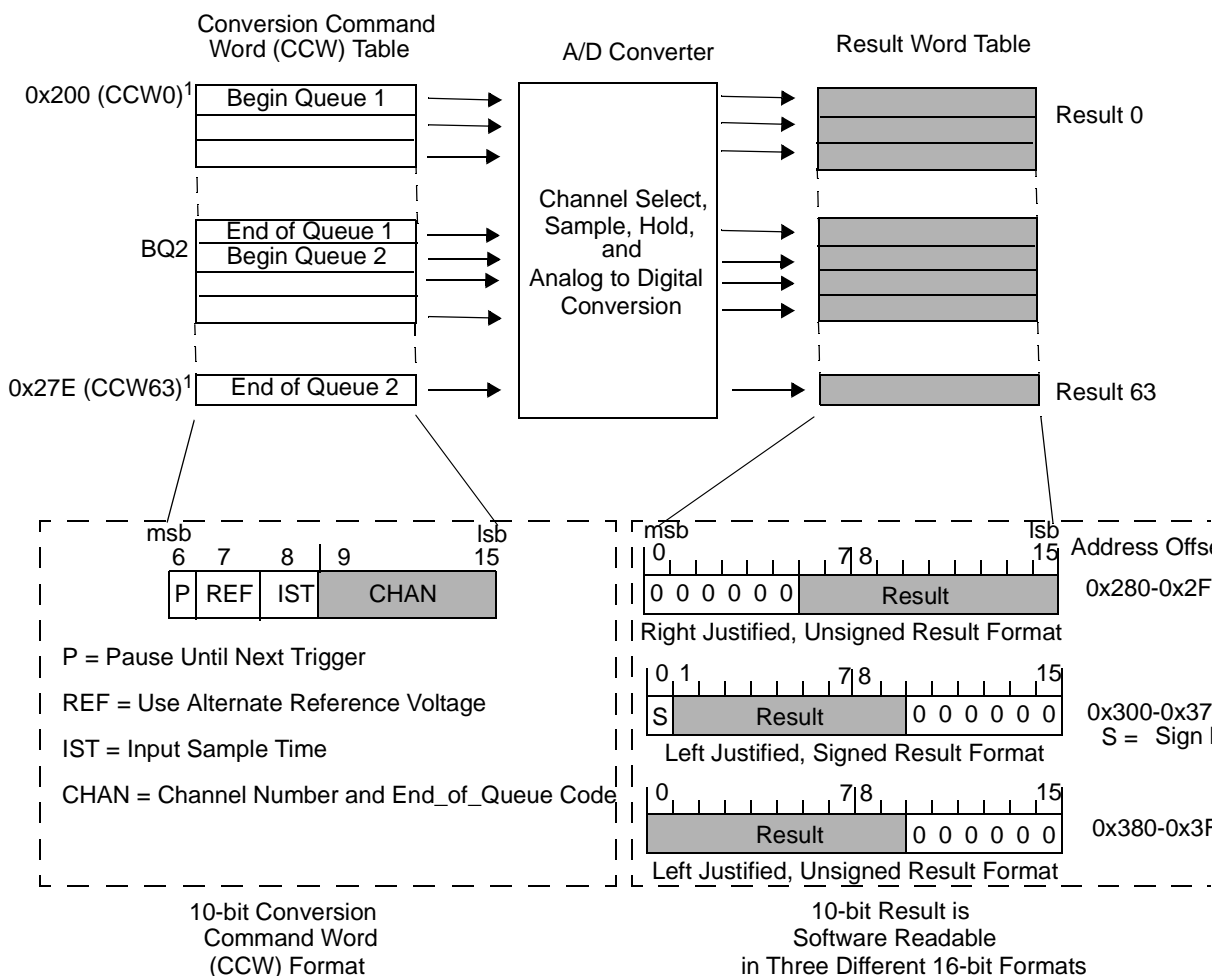
Figure 14-15. QADC64E Conversion Queue Operation
