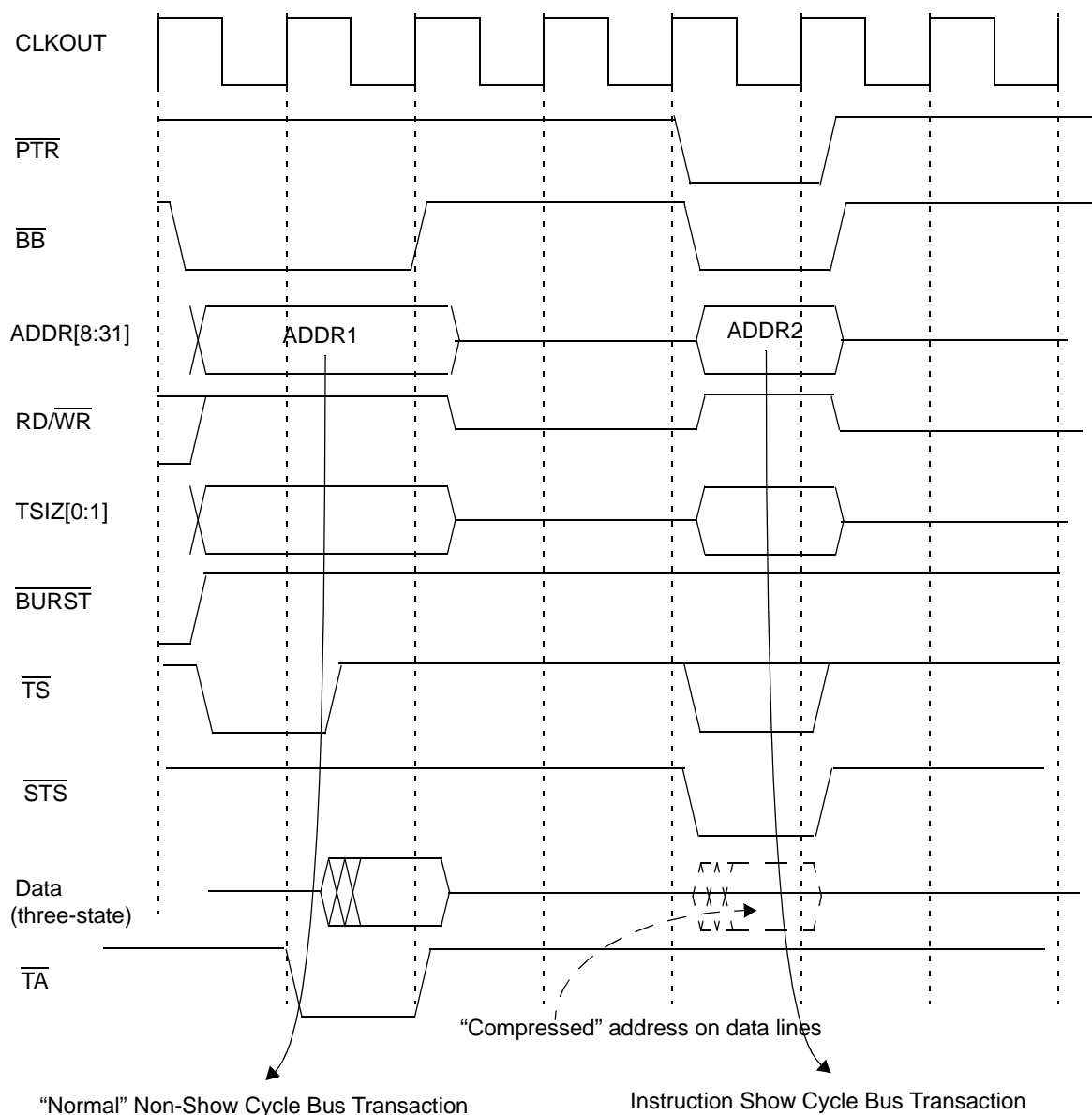
Figure 9-41. Instruction Show Cycle Transaction
