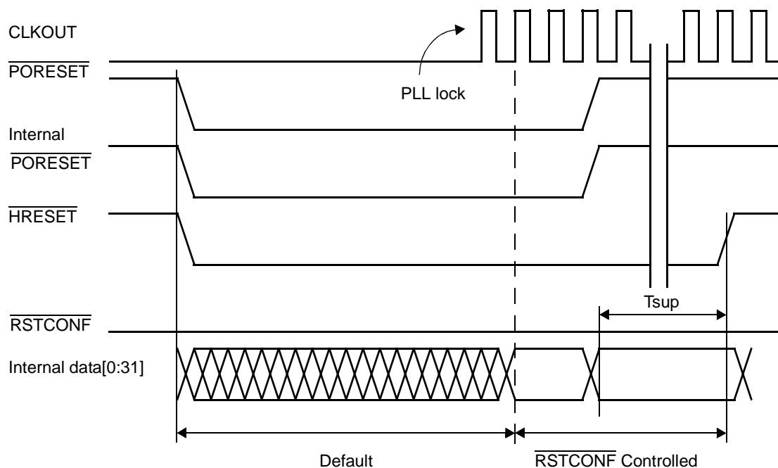
Figure 7-5. Reset Configuration Timing for “Long” \overline{\text{PORESET}} Assertion, Limp Mode Disabled
