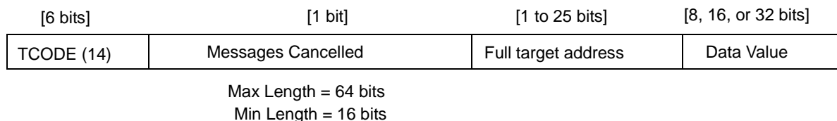
Figure 24-47. Data Read Synchronization Message Format
