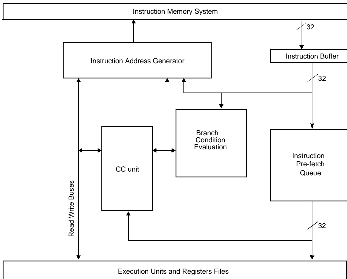
Figure 3-2. Sequencer Data Path
