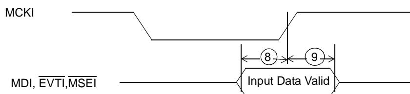
Figure G-29. Auxiliary Port Data Input Timing Diagram
