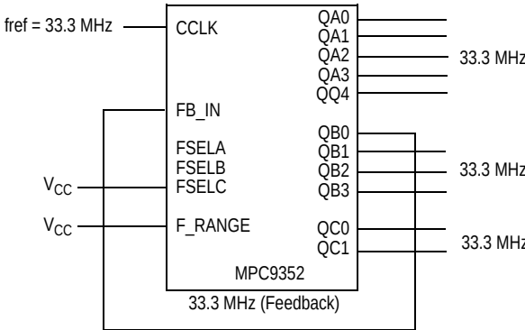
MPC9352 zero-delay (feedback of QB0 = 33.3 MHz). Equivalent to Table 2 except F_RANGE = 1 enabling a lower input and output clock frequency.
