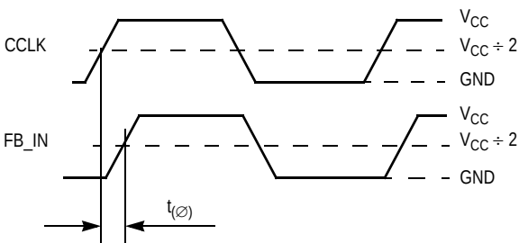
Figure 15. Propagation Delay ( t_{(0)} , static phase offset) Test Reference
