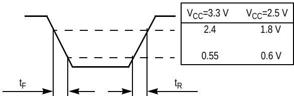
Figure 20. Output Transition Time Test Reference
