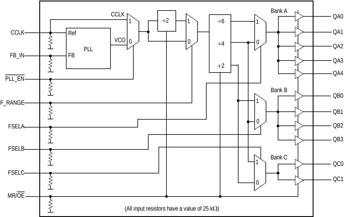
Figure 1. MPC9352 Logic Diagram
