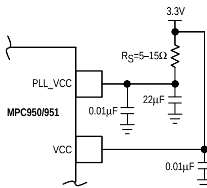
Figure 10. Power Supply Filter
