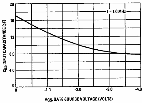
FIGURE 3 - INPUT CAPACITANCE
