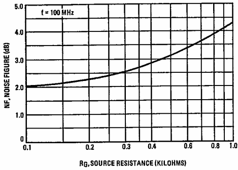
FIGURE 1 - NOISE FIGURE
