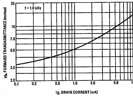
FIGURE 2 - FORWARD TRANSADMITTANCE
