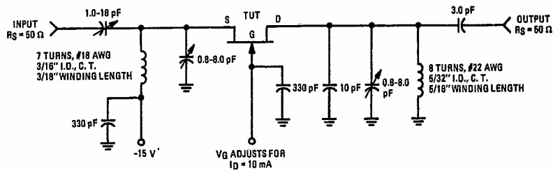
FIGURE 5 - 100 MHz TEST CIRCUIT
