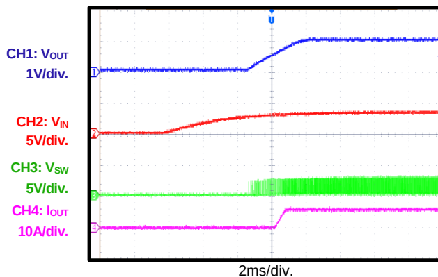
V_{IN} Start-Up
