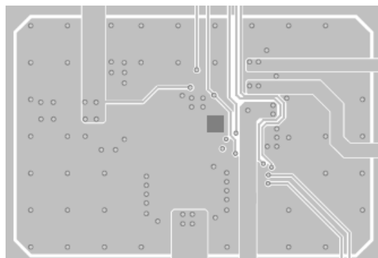
Mid-Layer 2
