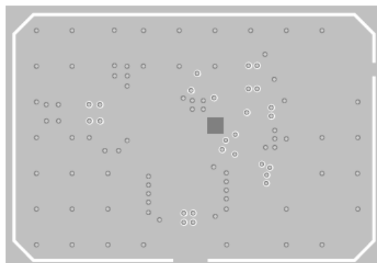
Mid-Layer 1
