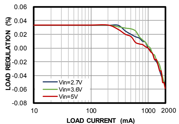
Load Regulation
