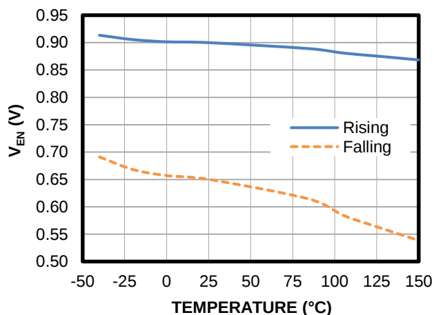
V_{EN} Rising and Falling Threshold vs. Temperature
