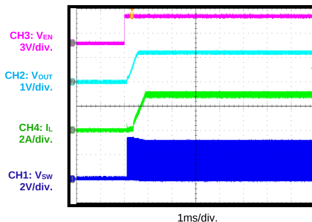
Start-Up through EN
