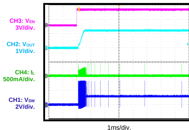
Start-Up through EN
