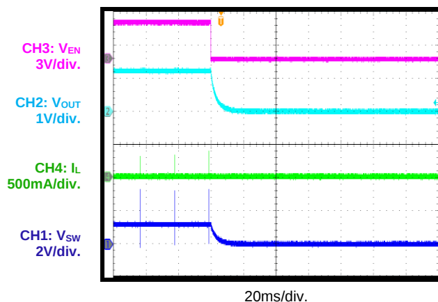
Shutdown through EN
