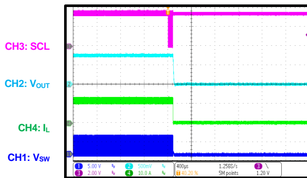
Shutdown via the Digital Interface I_{OUT} = 12A
