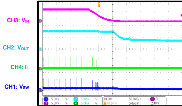
Shutdown through VIN I_{OUT} = 0A , DCM
