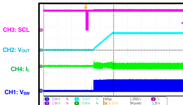
Start-Up via the Digital Interface
