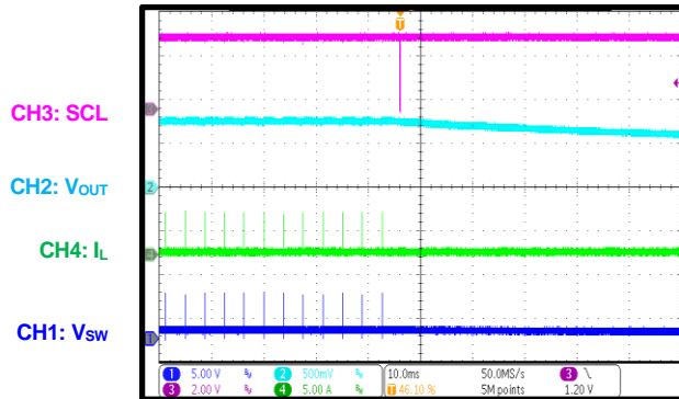
Shutdown via the Digital Interface I_{OUT} = 0A , DCM
