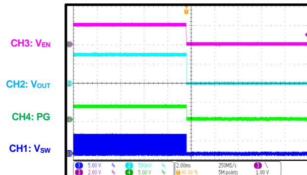
PG during Shutdown through EN I_{OUT} = 12A
