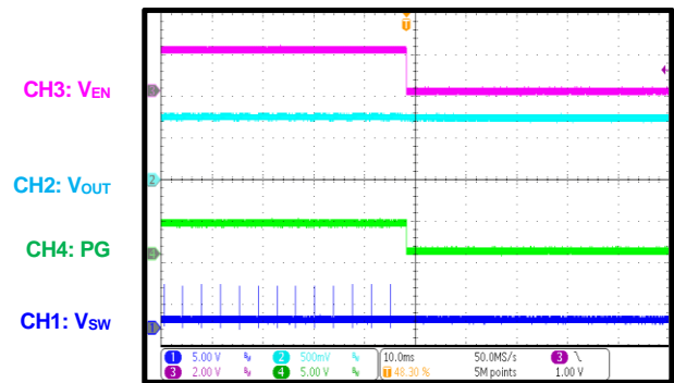
PG during Shutdown through EN I_{OUT} = 0A , DCM
