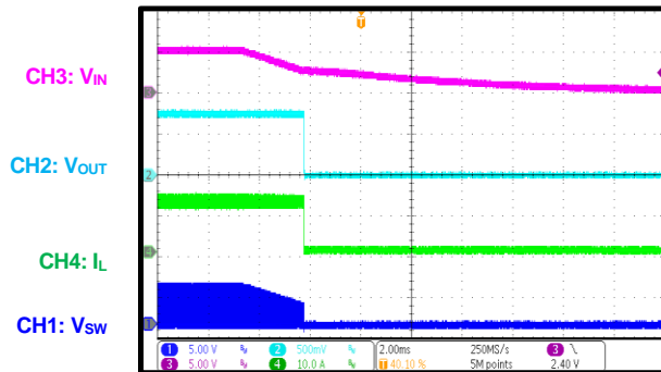
Shutdown through VIN I_{OUT} = 12A
