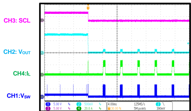
SCP Entry I_{OUT} = 0A , DCM
