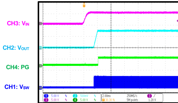
PG during Start-Up through VIN I_{OUT} = 12A
