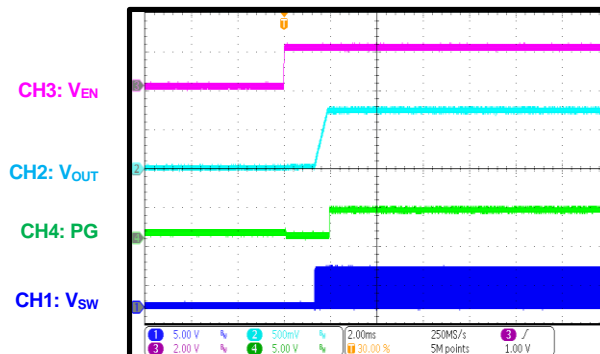
PG during Start-Up through EN I_{OUT} = 12A
