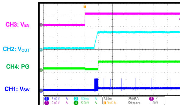
PG during Start-Up through EN I_{OUT} = 0A , DCM
