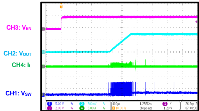
Start-Up through EN I_{OUT} = 0A , DCM
