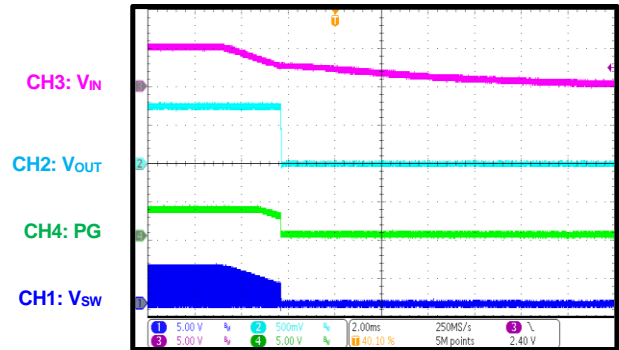
PG during Shutdown through VIN I_{OUT} = 12A
