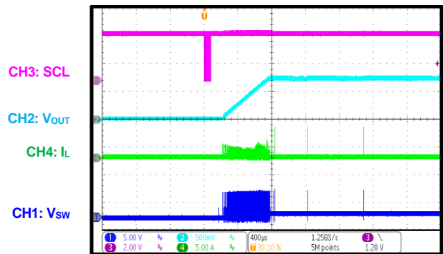
Start-Up via the Digital Interface
