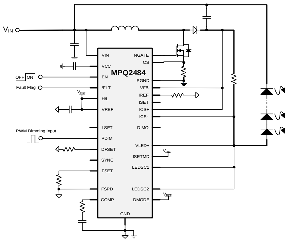
Figure 2: Buck-Boost Configuration
