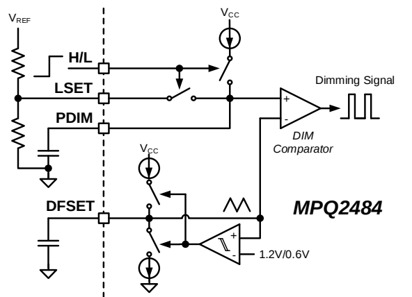
Figure 7: Two-Step Dimming
