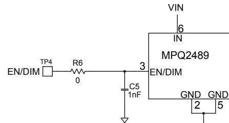
Figure 2—Analog Dimming External Circuit
