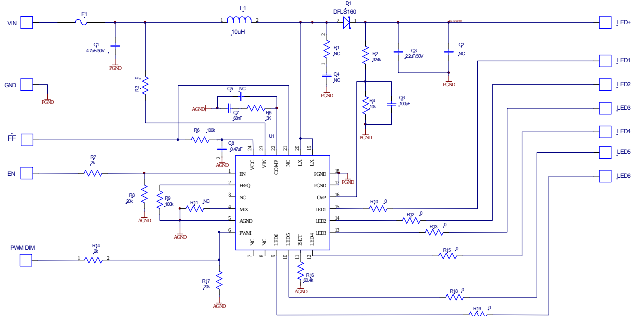
Figure 1: V_{IN} > 5.5V , 6string, 20mA/string application (Some components are reasonably adjustable based on real case)
