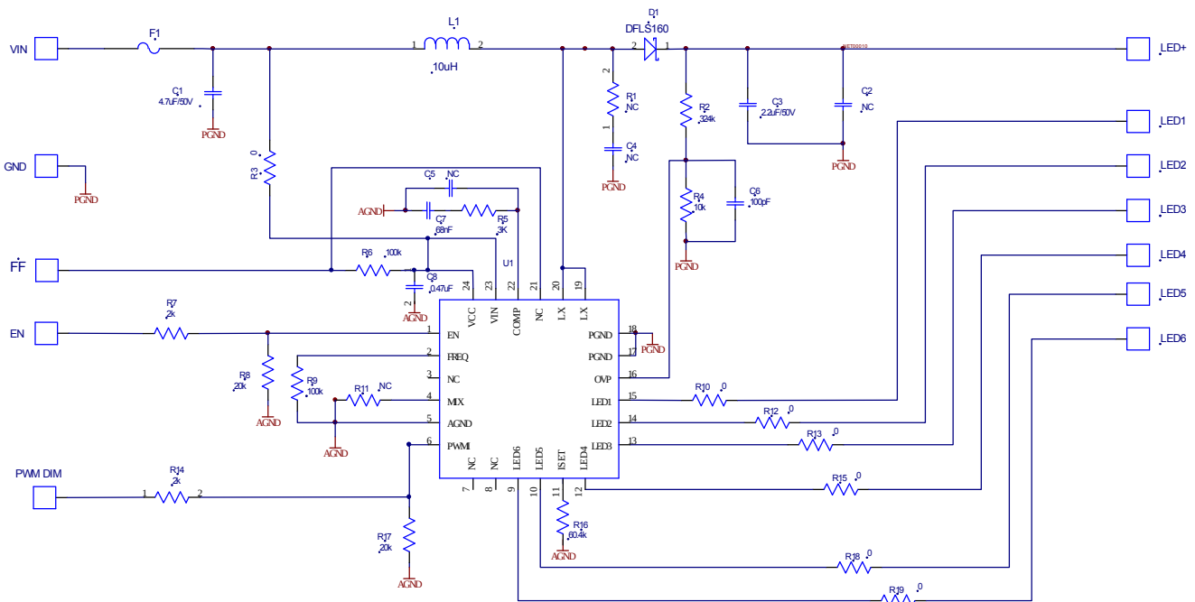
Figure 2: V_{IN} < 5.5V , 6string, 20mA/string application (Tie VIN and VCC together, some components are reasonably adjustable based on real case)
