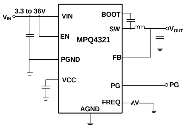
Figure 2: Fixed Output
