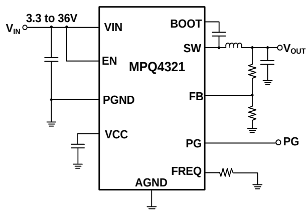
Figure 1: Adjustable Output
