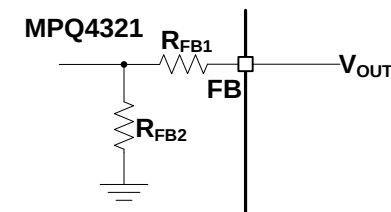
Figure 9: Feedback Divider Network (Fixed Output)
